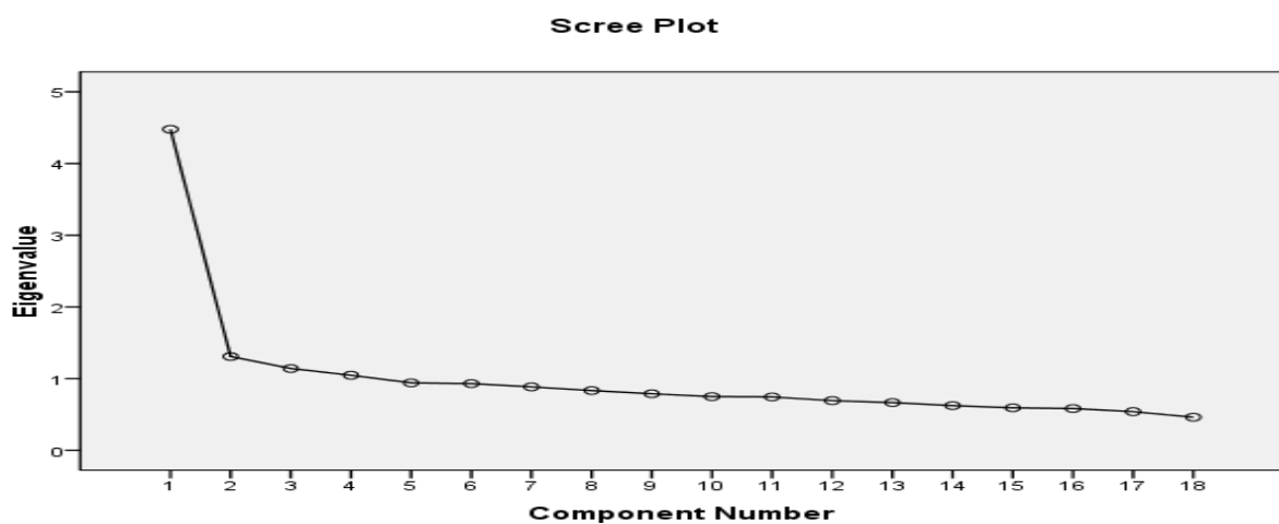
Fig. 1 showing the graphical representations of the item's wise eigenvalue
